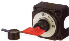
OVER- and UNDER MOUNT. MAIN SWITCH with 2 keys Waterprotected. 250 / 350 amp.
